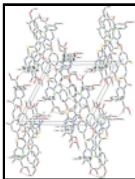
Fig. 2. The crystal packing of the title compound, viewed along the a axis. H atoms not involved in the intermolecular interactions (dashed lines) have been omitted for clarity.
